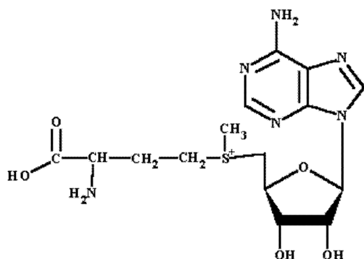
Fig. 1. Chemical structure of the SAM molecule.
