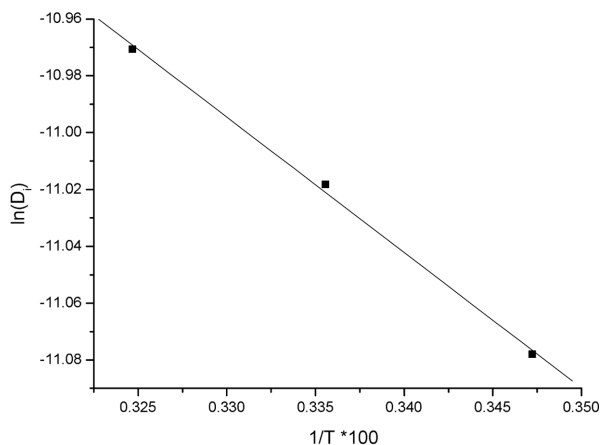
Fig. 11. The effect of temperature on intra-particle diffusivity.
